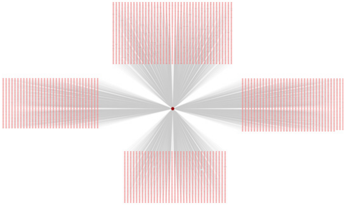
Figure 2. ALS-targets network.
