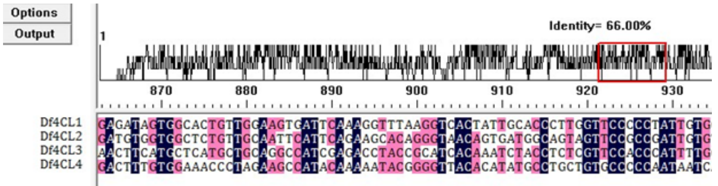
Supplementary Figure 2. Comparison of amino acid sequences of 4CL gene family of D. fragrans .
