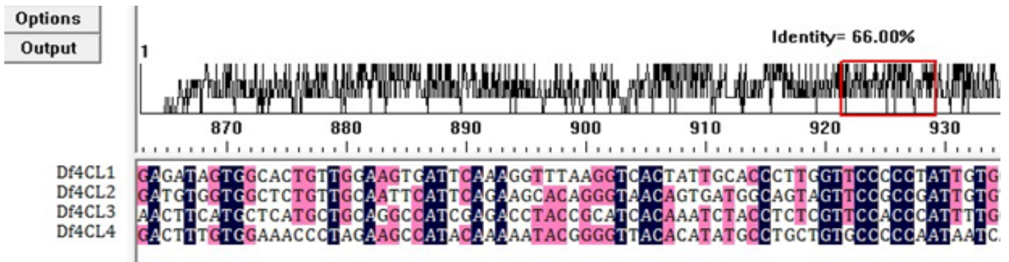
Supplementary Figure 1. Comparison of nucleic acid sequence of 4CL gene family of D. fragrans .
